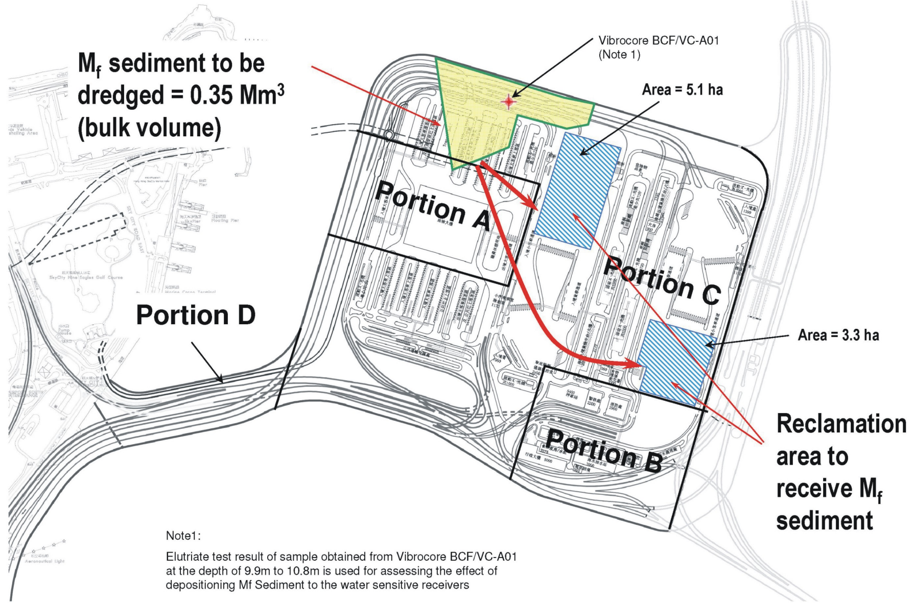
Figure 9 - Location Plan for the Two Pits to Receive M_f Sediment in HKBCF
